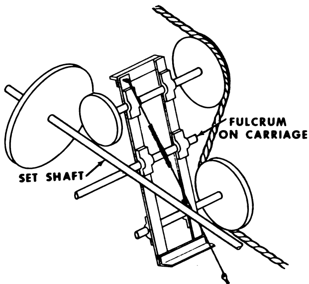
Figure 8-20. Fixed-rope, friction-wheel type of power setworks.
